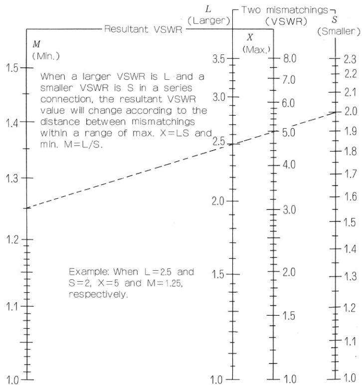
Max. and Min. VSWR Values Caused by Two Mismatchings
