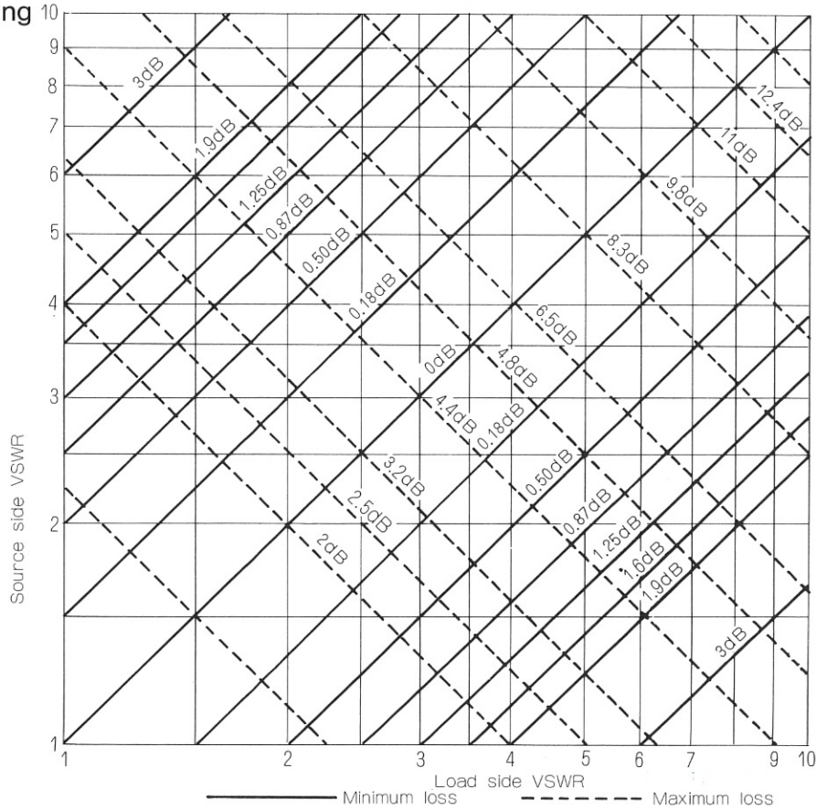
Max. and Min. VSWR Values Caused by Two Mismatchings
